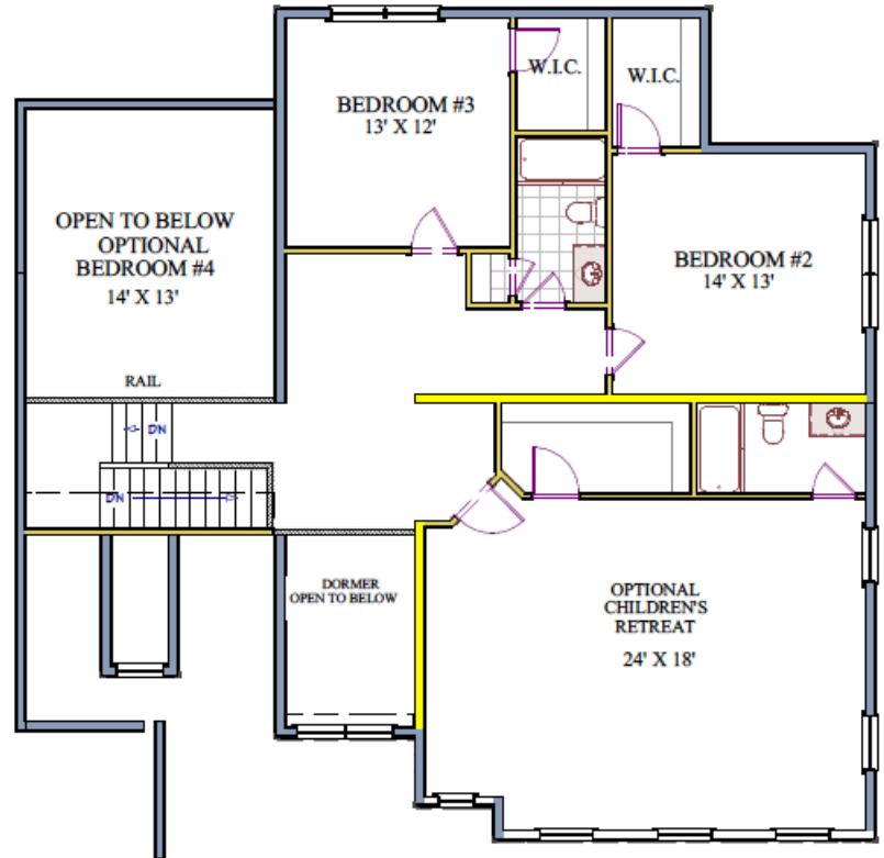
Optional 2 nd Floor Plan
