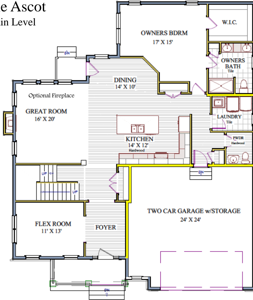
Optional 4' extension to owner BDRM
