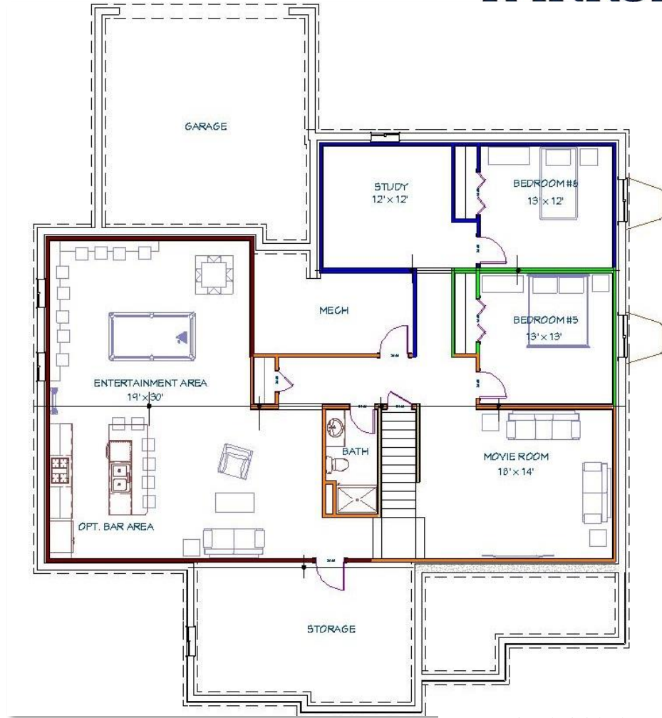
Optional Finished Basement
