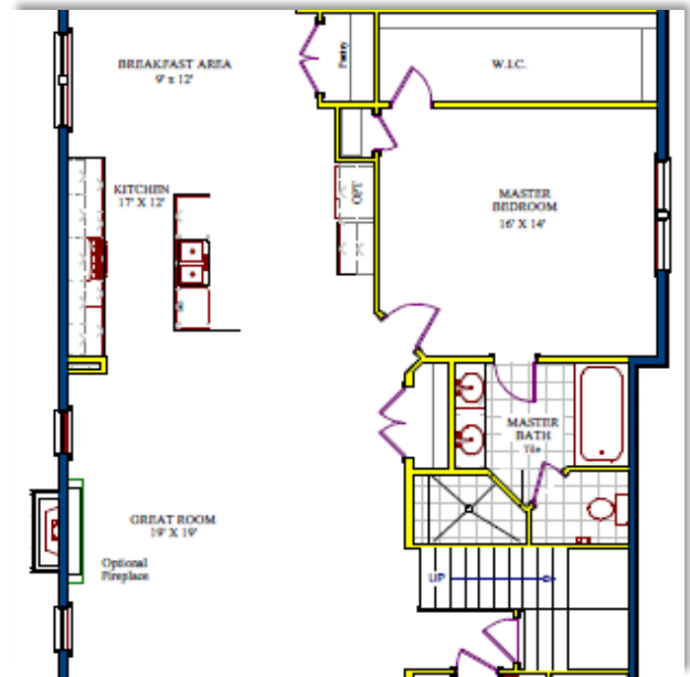
Optional Owner Bath with Soaking Tub & Shower
