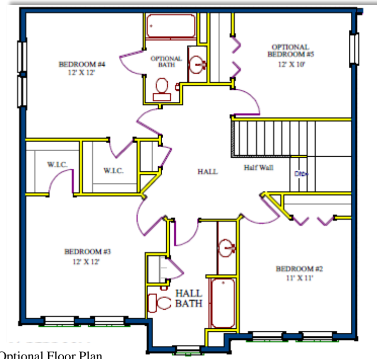
Optional Floor Plan With 5BR Guest Suite
